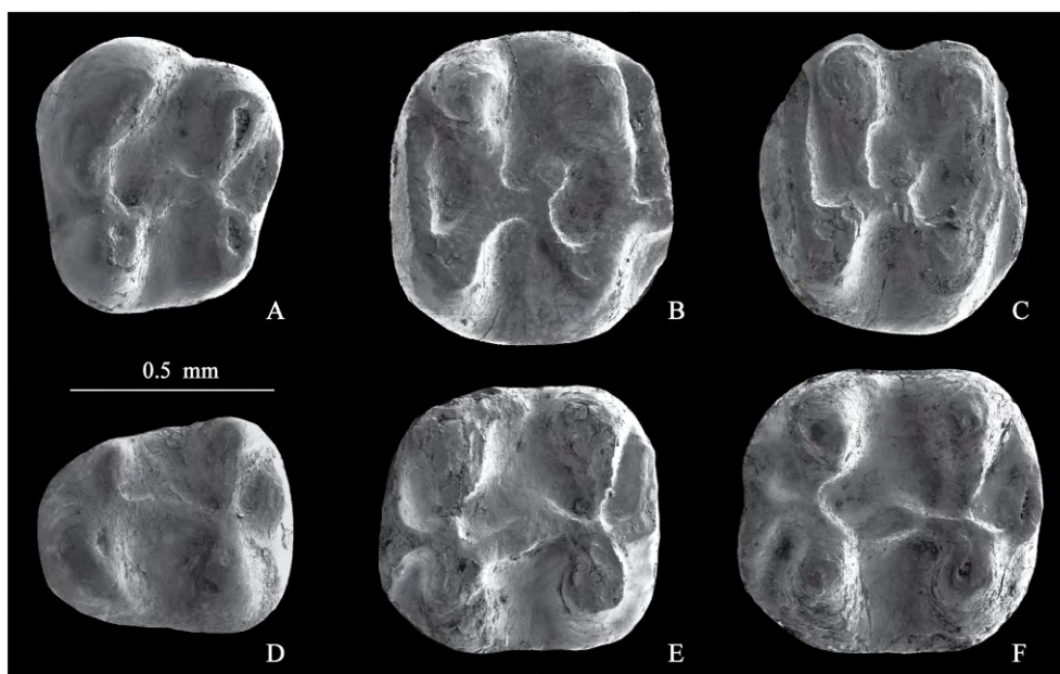
Fig. 3 Cheek teeth of Yuneomys pusillus from Lufeng, Yunnan in occlusal views A. 1 P4 (IVPP V 14733.4); B. r M1/2 (V 14732, holotype, reversed); C. r M1/2 (V 14733.1, reversed); D. 1 p4 (V 14733.5); E. 1 m1/2 (V 14733.2); F. 1 m1/2 (V 14733.6)
