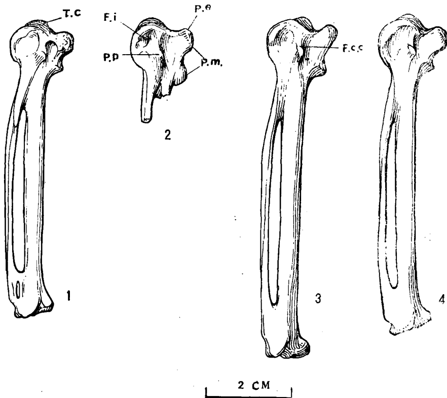
图 2A 鸛科鸟类左腕掌骨对比。内侧视, 1. 白鹮; 2. 天岗琵鹭新种; 3. 大琵鹭; 4. 朱鹮 Fig. 2A Comparison of the carpometacarpus of Threskionithidae 1. Threskionis aethiopicus ; 2. Platalea tinangensis sp. nov.; 3. Platalea leucorodia ; 4. Nippona nippon . internal view
