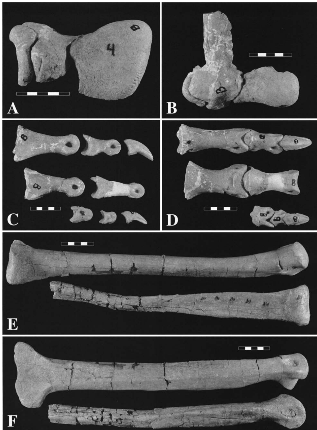
FIGURE 1. Cf. Ornithomimidae gen. et. sp. indet., IVPP V12756. A , B , right astragalus and calcaneum in (A) distal and (B) extensor views. Extensor side is at top in A . C , D , three phalanges of digit II (top row), first and second phalanges of digit III (middle row), and third through fifth phalanges of digit IV (bottom row) in (C) lateral and (D) extensor views. E , F , metatarsal II (top) and metatarsal III (bottom) in (E) extensor and (F) lateral views. Scale bars equal 5 cm.
