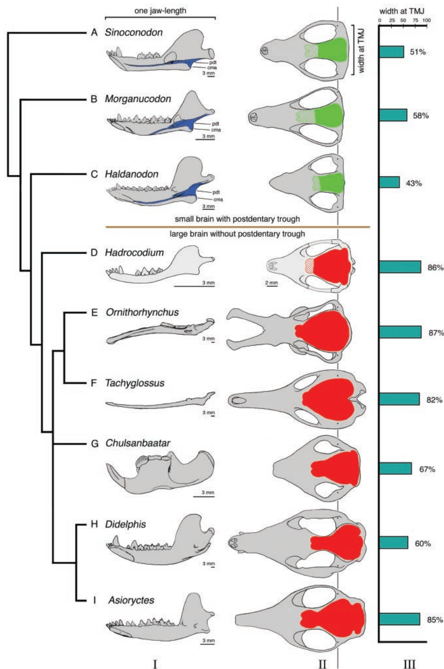
Fig. 3. Correlation of the expanded brain vault and the loss of the postdentary trough and medial concavity of mandibular angle in Hadrocodium and more derived mammals. (I, Left) Internal view of dentaries (standardized to one jaw length, scales differ among taxa); the postdentary trough, the medial concavity, and the meckelian sulcus on the mandibular angle are colored in blue. Abbreviations: cma, medial concavity of the mandibular angle; pdt, postdentary trough. (II, Middle) Dorsal view of the cranium (crania of different sizes are standardized to the same width between the left and right temporomandibular joints; scales differ among taxa); the areas in red represent the approximate extent of the brain endocasts. (III, Right) Measurement of the brain vault size (cranial width at the squamosal-parietal suture) relative to the width between the two TMJs; value on bar represents the width of brain vault in percentage of total skull width at the TMJs. Hadrocodium (85%) and mammalian crown groups (60% to 87%) with larger brain vaults show the separation of the middle ear ossicles from the mandible. Hadrocodium has a larger brain vault than expected for living mammals of its skull size (see allometry regression in Fig. 5B) and is similar to living mammals but different from other contemporaneous mammaliaforms. All primitive mammaliaforms [(A) to (C)] in the basal part of the tree have the postdentary trough and medial concavity of mandibular angle (for postdentary "ear" elements), as well as small brain vault (43% to 58%). The 58% value for Morganucodon , although larger than Haldanodon and Sinoconodon , is far below the ~75% expected for extant mammals of similar skull size (Fig. 5A). (A) Sinoconodon . (B) Morganucodon . (C) Haldanodon [after (23)]. (D) Hadrocodium (brain endocast outline based on the exposed borders on the right side). (E) Monotreme Ornithorhynchus . (F) Monotreme Tachyglossus . (G) Multituberculate Chulsanbaatar [after (36)]. (H) Marsupial Didelphis [after (33)]. (I) Placental Asioryctes [after (31)].
