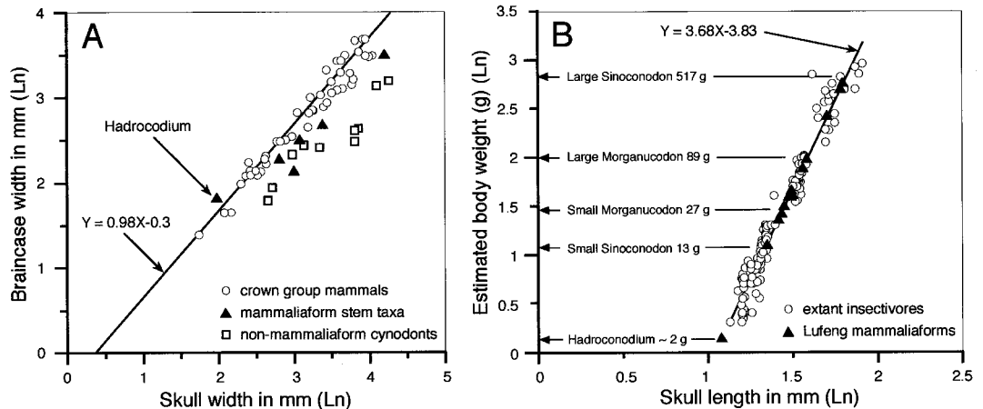
arily for comparison with the regression of extant and fossil species of mammalian crown group. (B) Estimated body-size distributions of mammaliaform insectivores in the Early Jurassic Lufeng fauna [following method of Gingerich (50)]. The estimated 2-g body mass of Hadrocodium is in strong contrast to its contemporary mammaliaforms of the Late Triassic and Early Jurassic, such as Sinoconodon (from ~13 to ~517 g, based on skull length from 22 to 62 mm) and Morganucodon (from 27 to 89 g, based on skull length from 27 to 38 mm). This wide range of body sizes indicates a trophic diversity in the paleoguild of triconodont-like insectivores (53, 54) in the Lufeng mammaliaform fauna.
