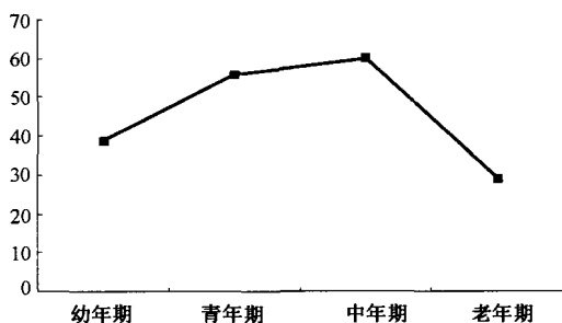
图 6 依据牙齿磨蚀阶段划分的田园洞梅花鹿死亡年龄结构 Age distribution of Cervus nippon at Tianyuan Cave, based on the attrition of teeth
