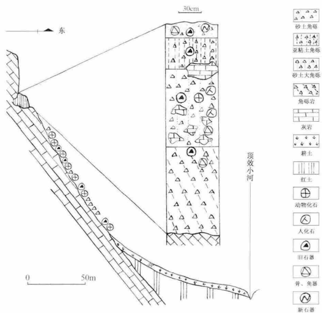
图 1 猫猫洞附近地貌示意图及遗址地层剖面图 Fig.1 The geomorphology schematic and stratigraphic section figure of Maomao cave
